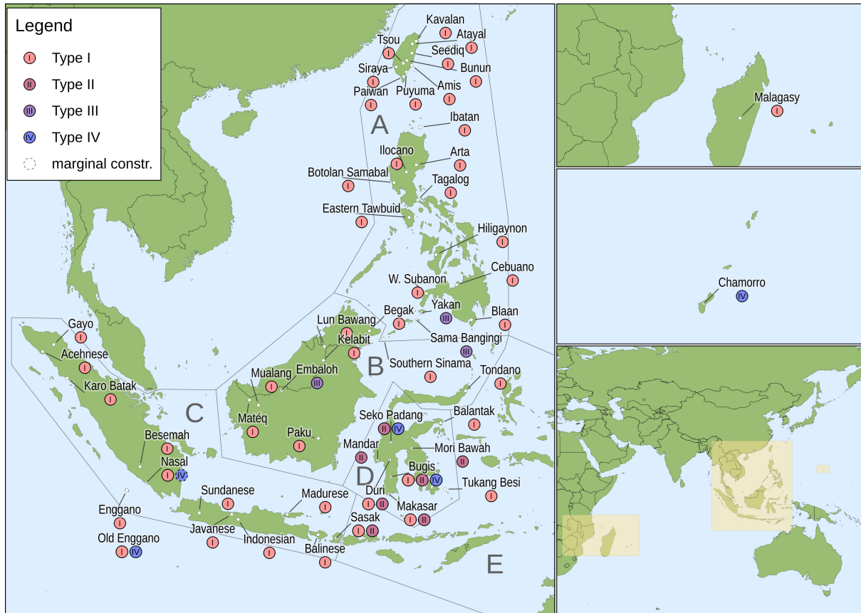
Figure 6: Distribution of Type I–IV constructions
