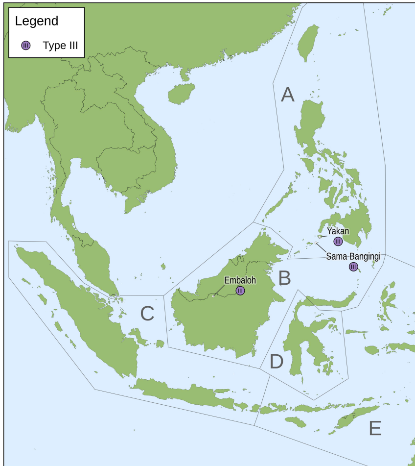
Figure 4: Distribution of Type III constructions
