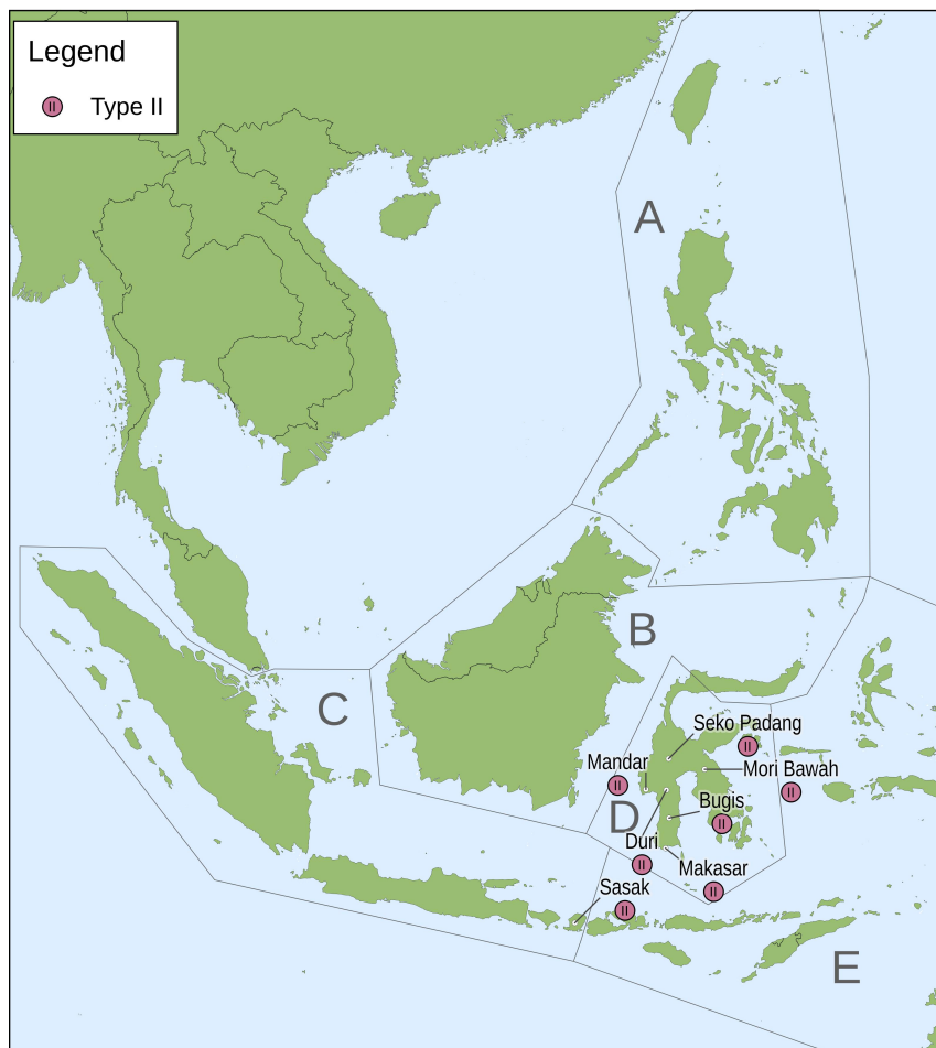
Figure 3: Distribution of Type II constructions
